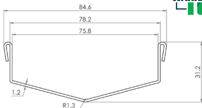
Profile
