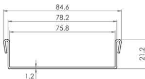
Profile
