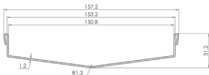
Profile
