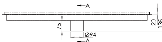
Front
