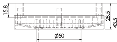
Cross Section
