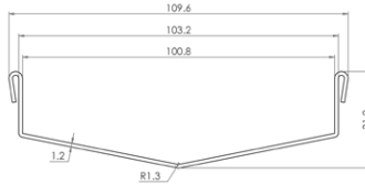
Profile
