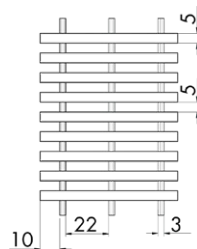
Grate
