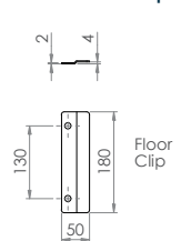
Floor Clip
