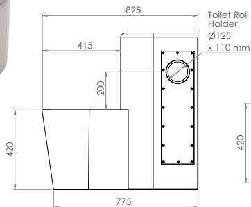
P Trap
