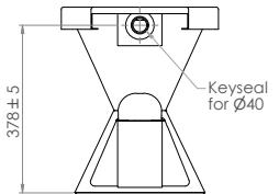
Floor Clip
