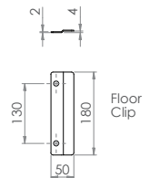
Floor Clip
