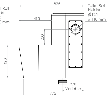
S Trap
