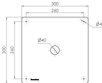
Face Plate 1.5mm 304 Grade Stainless Steel
