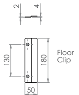
Floor Clip
