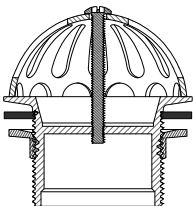
Section View on A - A
