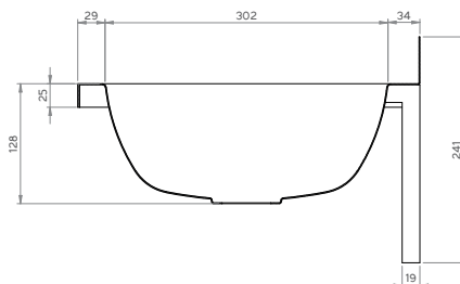
Section View on A - A
