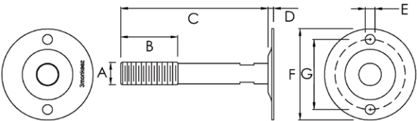
304 Grade Stainless Steel Adjustable Disc Foot
