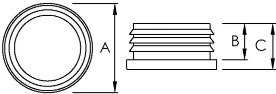
Plastic Tube Closure - Round Tube
