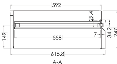
Cross Section
