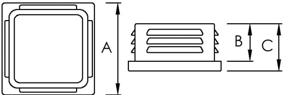
Plastic Tube Closure - Square Tube
