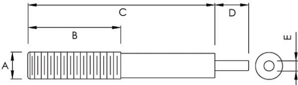
304 Grade Stainless Steel Adjustable Pin Foot
