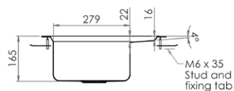
Section View on A - A
