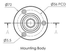
Mounting Body
