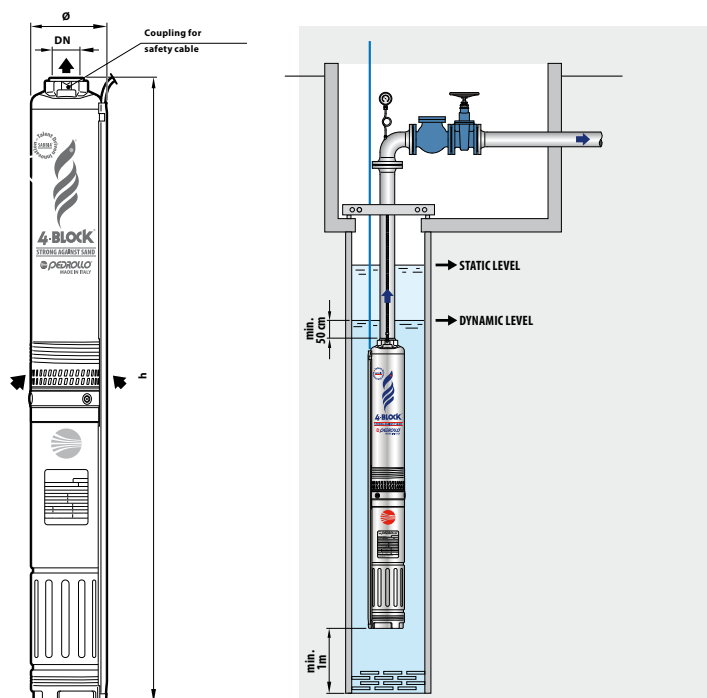
Typical installation
