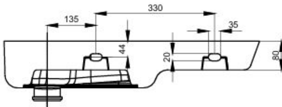
Back view
