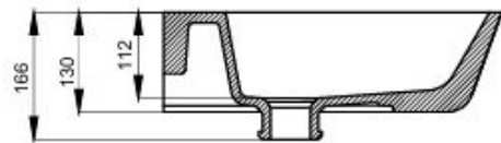
Section view
