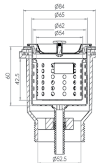
Cross Section
