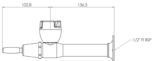
Side
